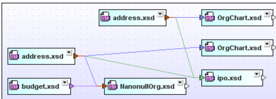
Hierarchical layout
