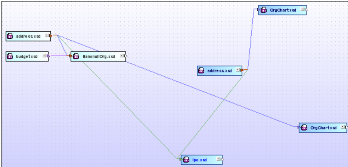
Force-directed layout
